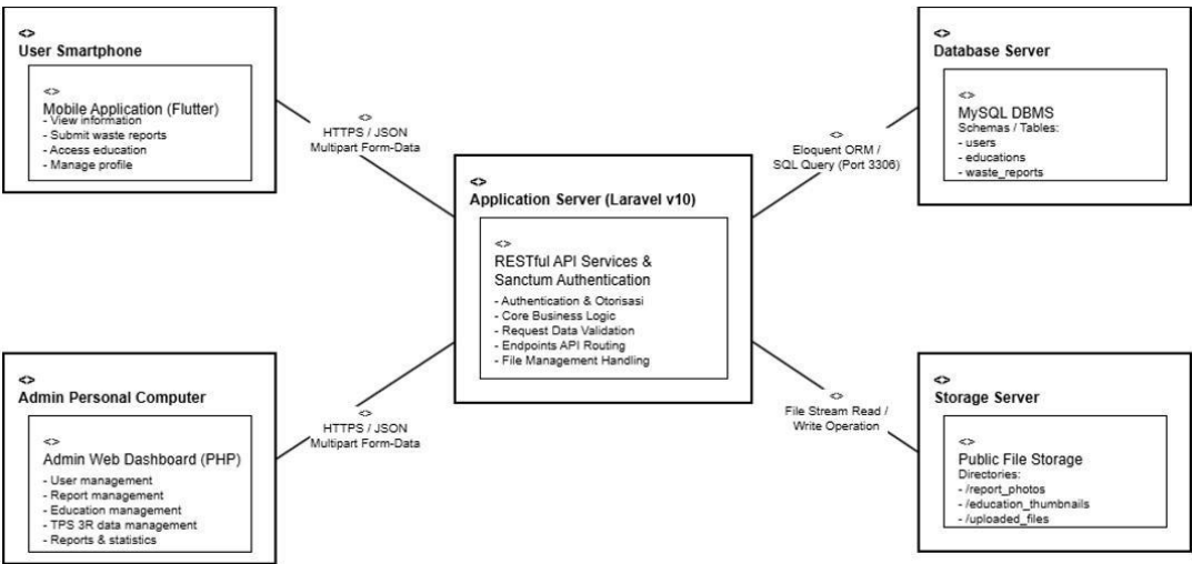
Gambar 1. Arsitektur Sistem Smart Waste Report
