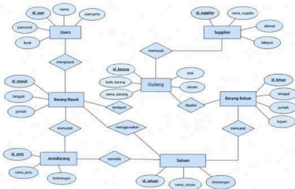
Gambar 7. Entity Relationship Diagram (ERD)
