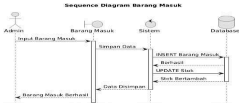
Gambar 5. Sequence Diagram Barang Masuk
