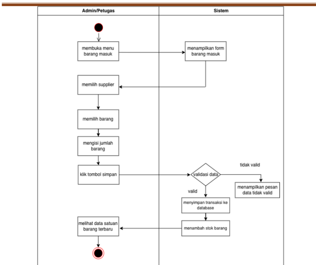
Gambar 4. Activity Diagram Barang Masuk
