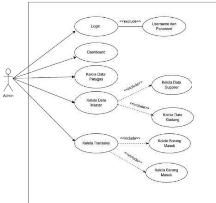
13 Gambar 2. Use Case Diagram Admin
