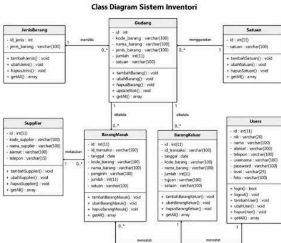
Gambar 6. Class Diagram
