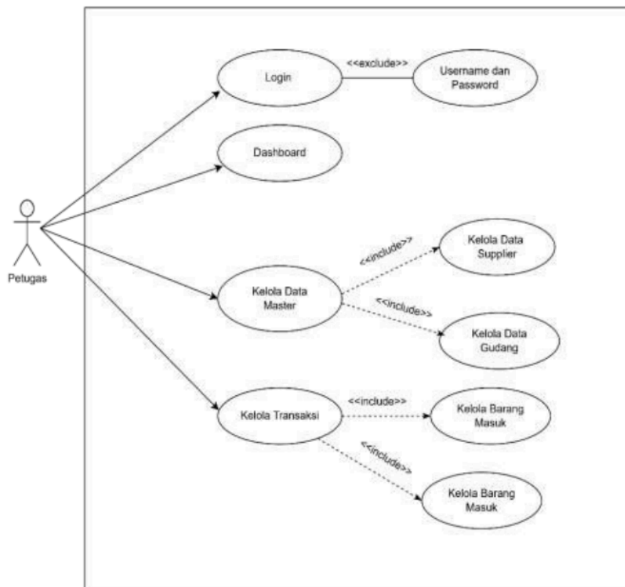
13 Gambar 3. Use Case Diagram Petugas
