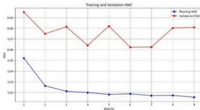
Gambar 6. Kurva Training dan Validation MAE Model LSTM
