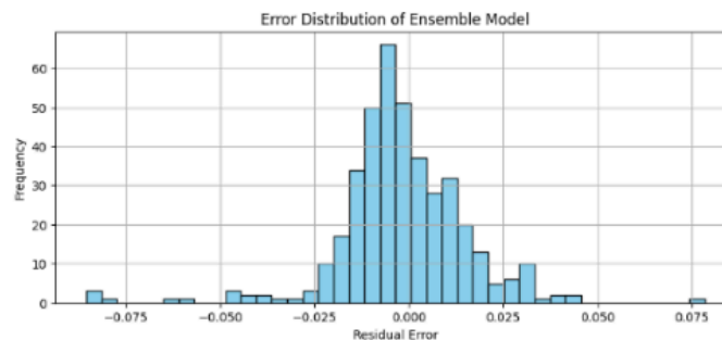
Gambar 9. Histogram Distribusi Error Ensemble
