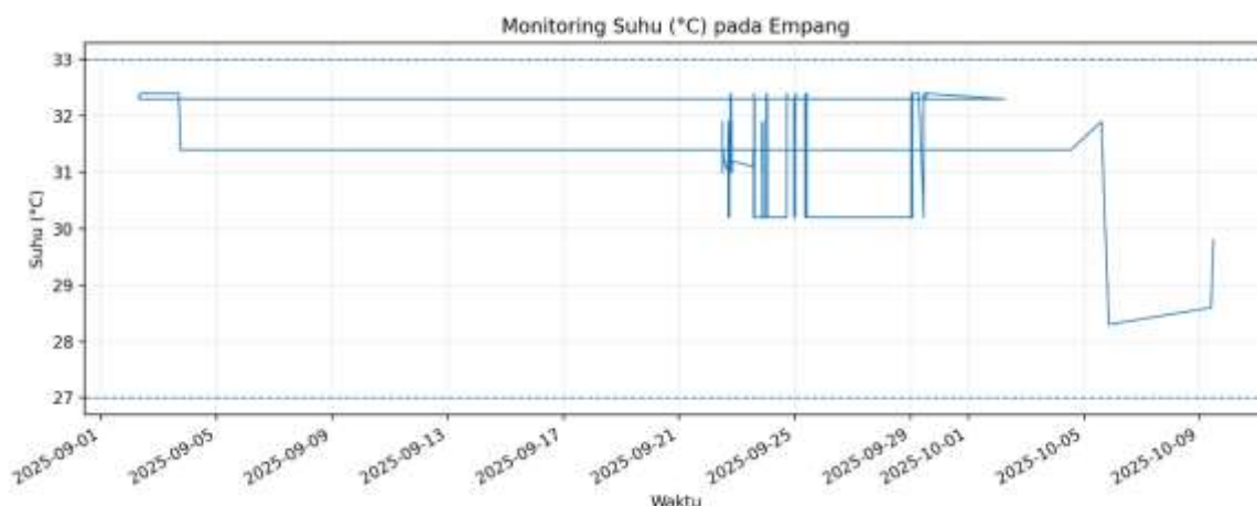
Gambar 6. Grafik Hasil Monitoring Suhu Air
