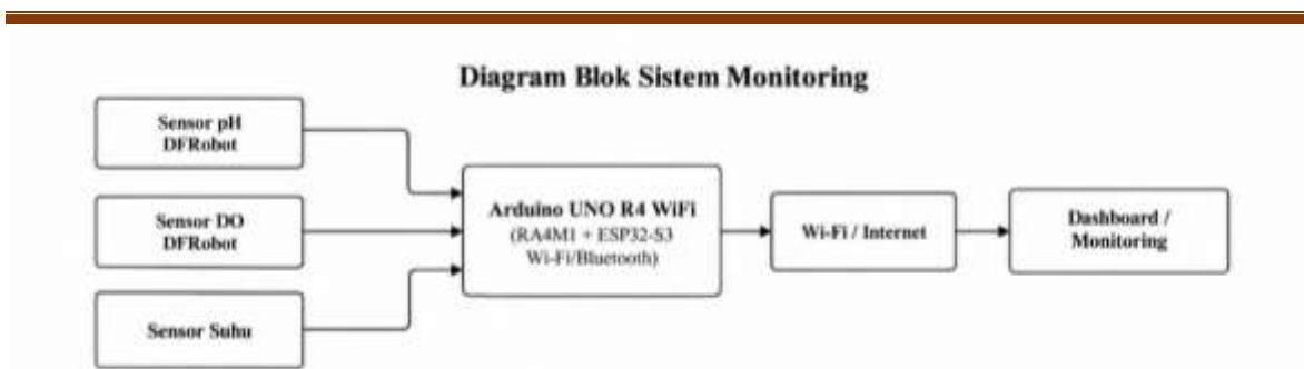
Gambar 2. Diagram Blok Sistem Monitoring
