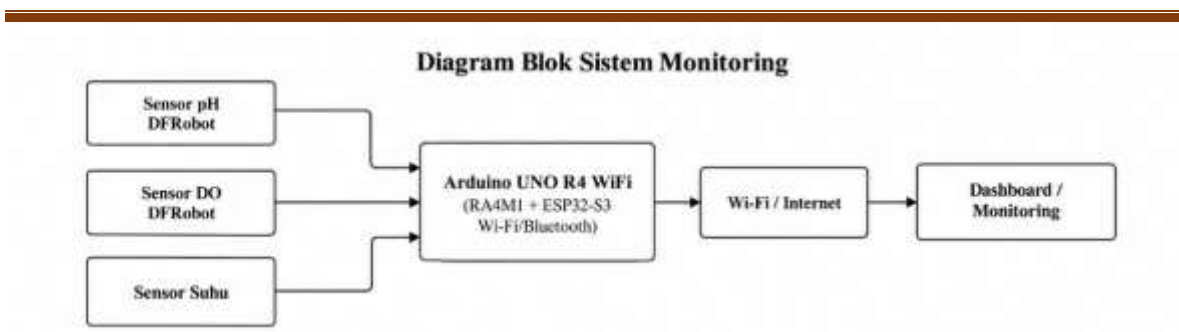
Gambar 3. Diagram Blok Sistem Monitoring Kualitas Air
