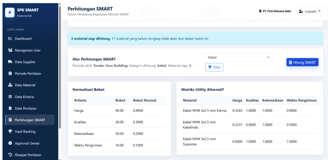
Gambar 7. Hasil Ranking
