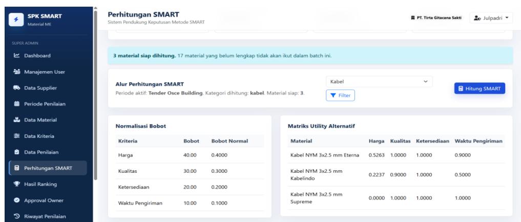
Gambar 6. Perhitungan SMART
