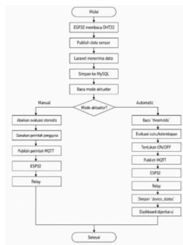
Gambar 2. Flowchart Kendali Hibrida
