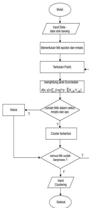
Gambar 3. Flowchart Algoritma Dbscan
