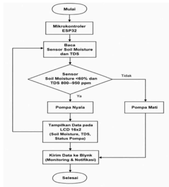
Gambar 3. Flowchart Sistem
