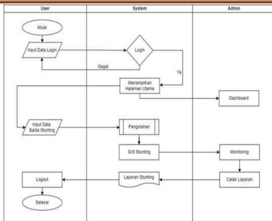
Gambar 2. Flowchart System
