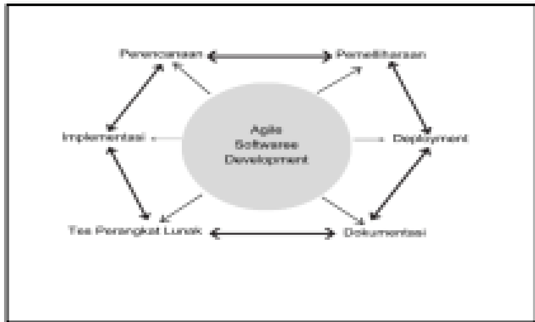
Gambar 1. Metode Agile
