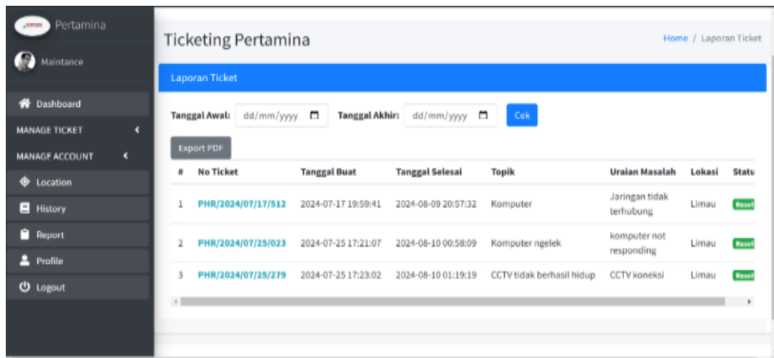
Gambar 18. Report
