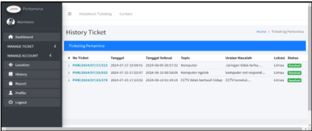
Gambar 17. History
