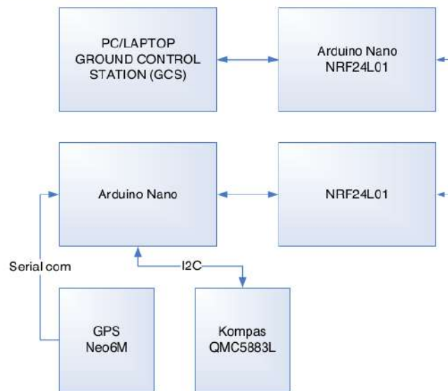
Gambar 1. Diagram Blok Umum Model Robot Mobil Beroda
