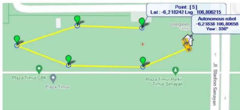
Gambar 11. Pengaturan 5 Waypoint
