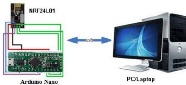
Gambar 5. Rancangan Perangkat Elektronik Ground Station
